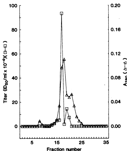
Fig. 3. Molecular sieve chromatography of the scrapie agent in sulfobetaine 3-14. Fraction P 5 was exposed to 10 percent (weight to volume) sulfobetaine 3-14 for 16 hours at 4°C and then chromatographed in 60 mM tris-acetate, pH 7.2 containing 1 mM EDTA and 0.024 percent sulfobetaine 3-14 over a molecular sieve (Toya Soda TSK 4000) column (0.75 cm, inside diameter, by 50 cm, length). The column was developed at 4°C (Varian 5000 HPLC) at 1 ml/min. Fractions (1 ml) were collected and assayed in hamsters by measurements of incubation time intervals. Blue dextran, bovine serum albumin, and tryptophan under identical conditions eluted in fractions 7, 15, and 22, respectively.
